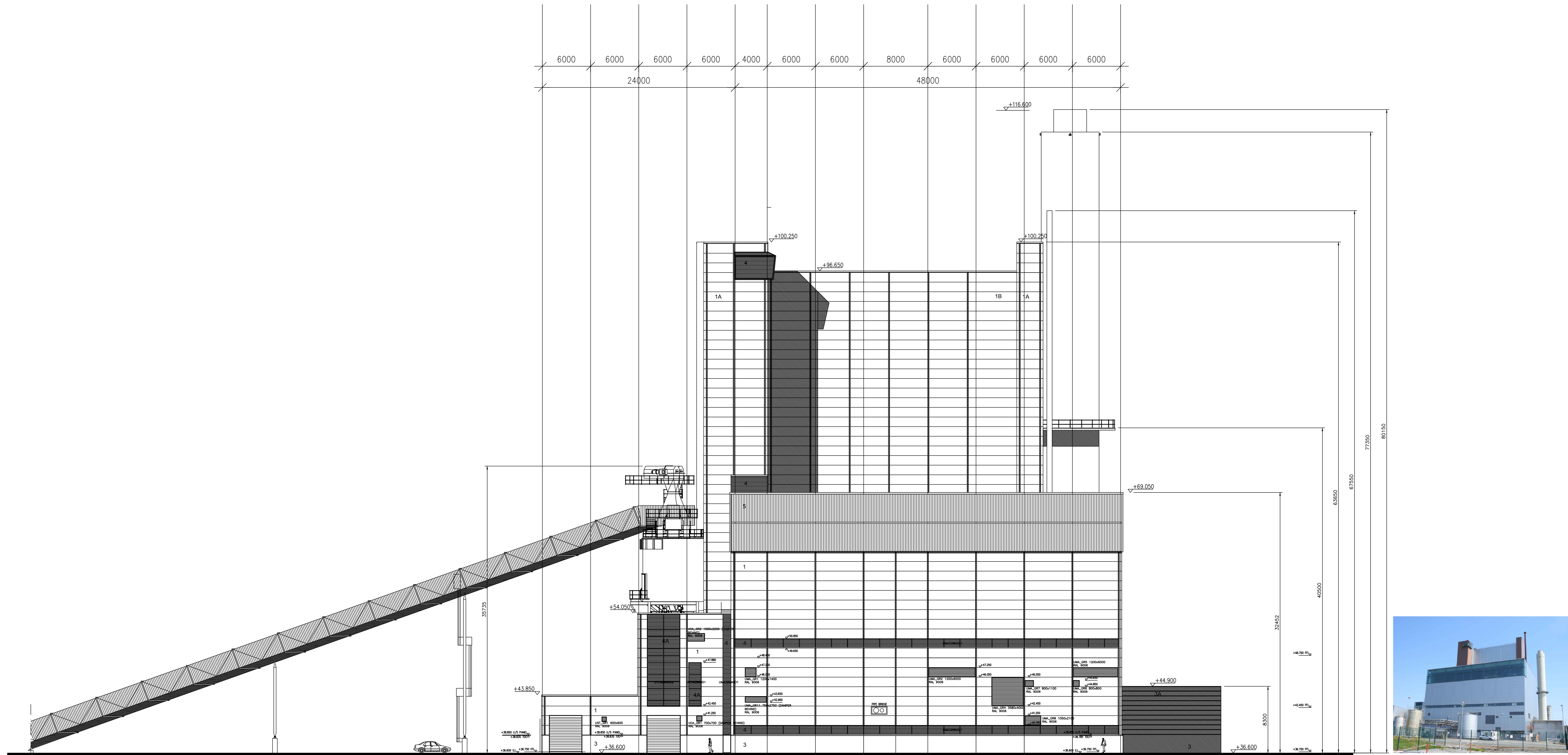
WEST ELEVATION
